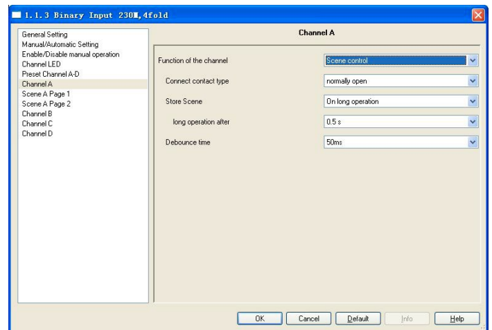
Fig.2.12 [1] Parameter window "Scene control, X"
