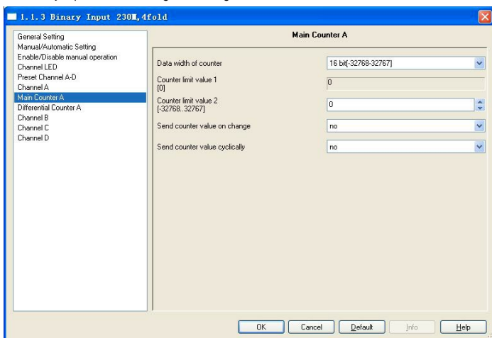
Fig.2.14 [2] Parameter window “Main Counter X”
