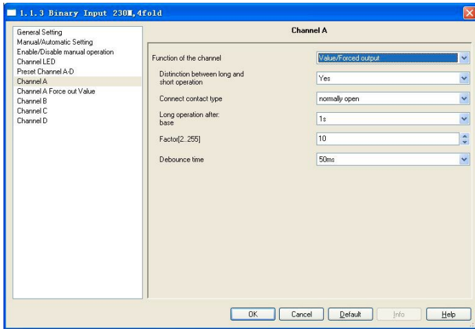
Fig.2.11[1] Parameter window "Value / Force output, X" (Distinction long/short operation)
