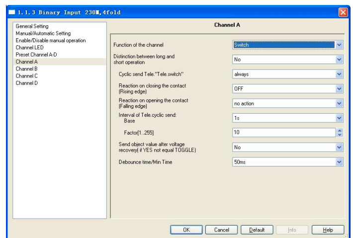
Fig.2.7 Parameter window "Switch" (No distinction long/short operation)
