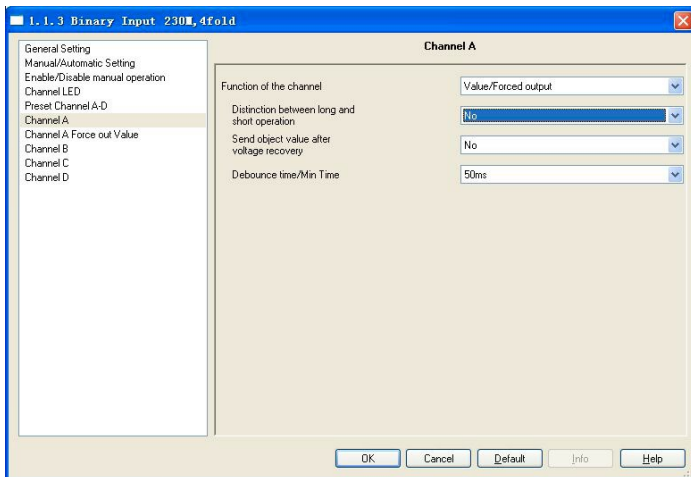
Fig.2.11[2] Parameter window "Value / Force output, X" (No distinction long/short operation)
