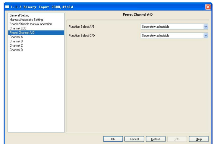
Fig.2.5 (1) Parameter window "Preset Channel A-D" [separately adjustable working mode]
