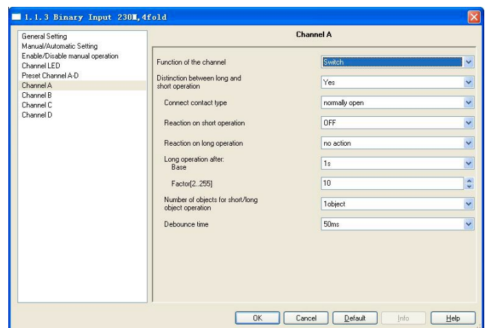
Fig.2.9 Parameter window "Switch" (Distinction long/short operation)
