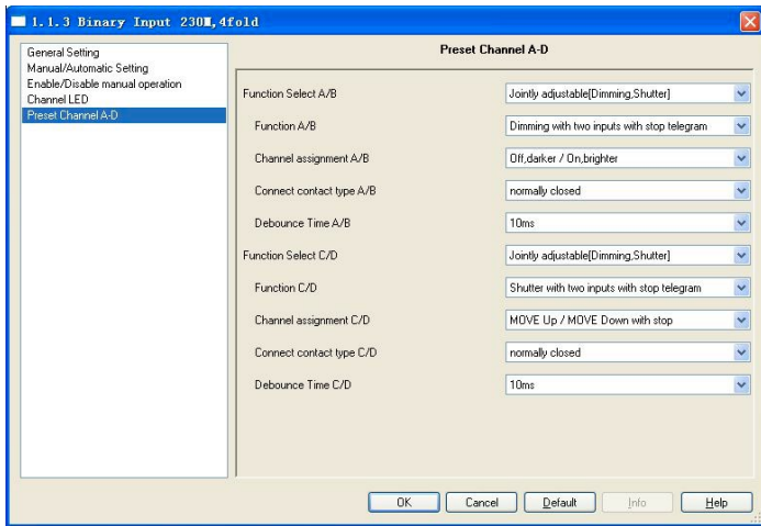
Fig.2.5 (2) Parameter window "Preset Channel A-D" [Jointly adjustable working mode]
