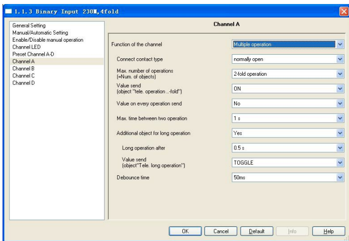
Fig.15 Parameter window “Multiple operation, X”
