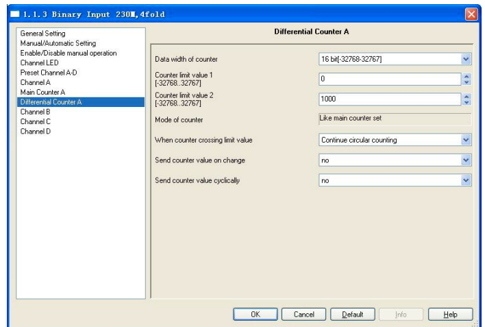
Fig.2.14[3] Parameter window “Differential Counter X”
